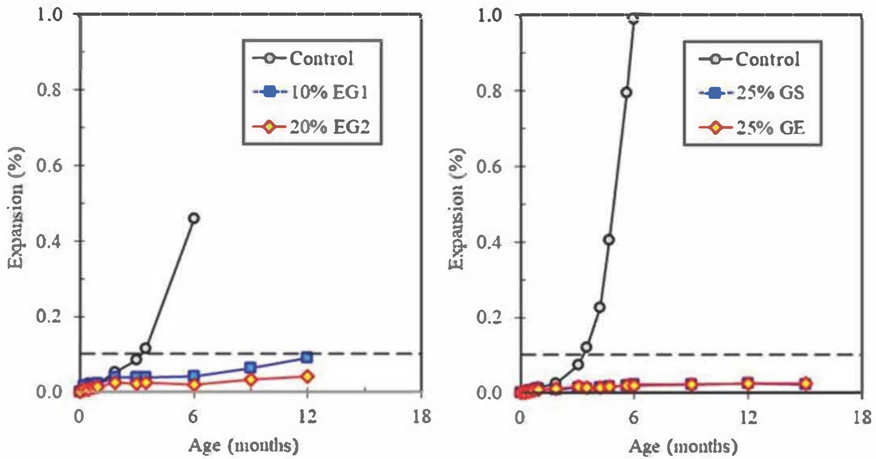
Figure 11 Improved Sulfate Resistance Evaluation of sulfate resistance testing for Type GS and Type GE Glass Pozzolans per ASTM C1012. Courtesy Mike Thomas.
