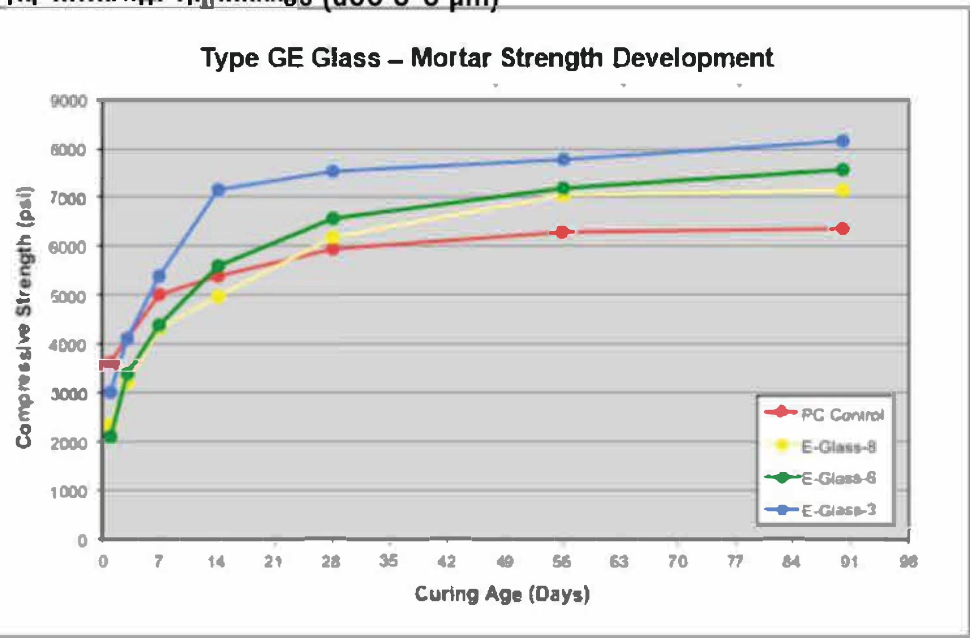
Type GE Glass: Strength development and strength activity index (SAI) for different finenesses (d50 3-8 \mu\text{m} )
