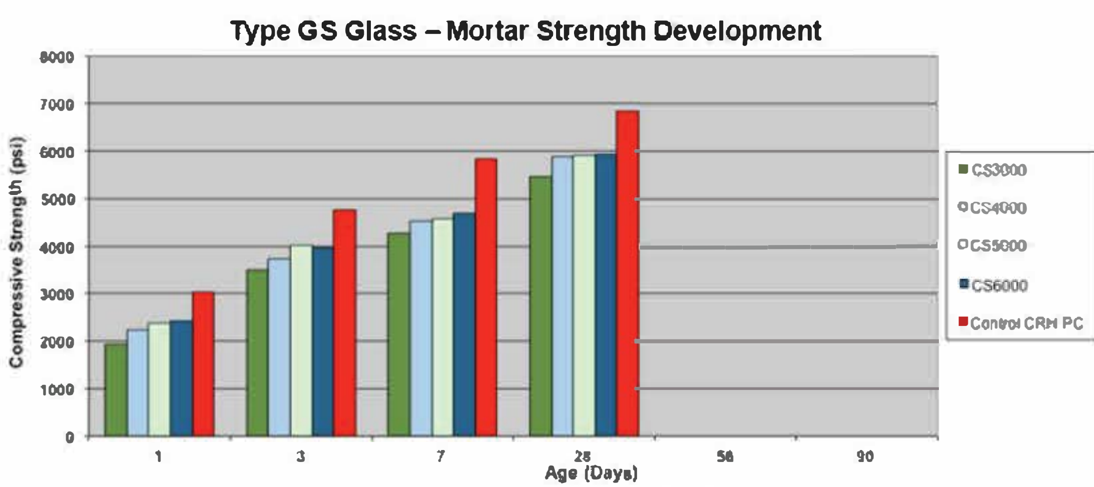
Type GS Glass: Strength development and strength activity index (SAI) for different Blaine finenesses (3,000-6,000 \text{cm}^2/\text{g} )
